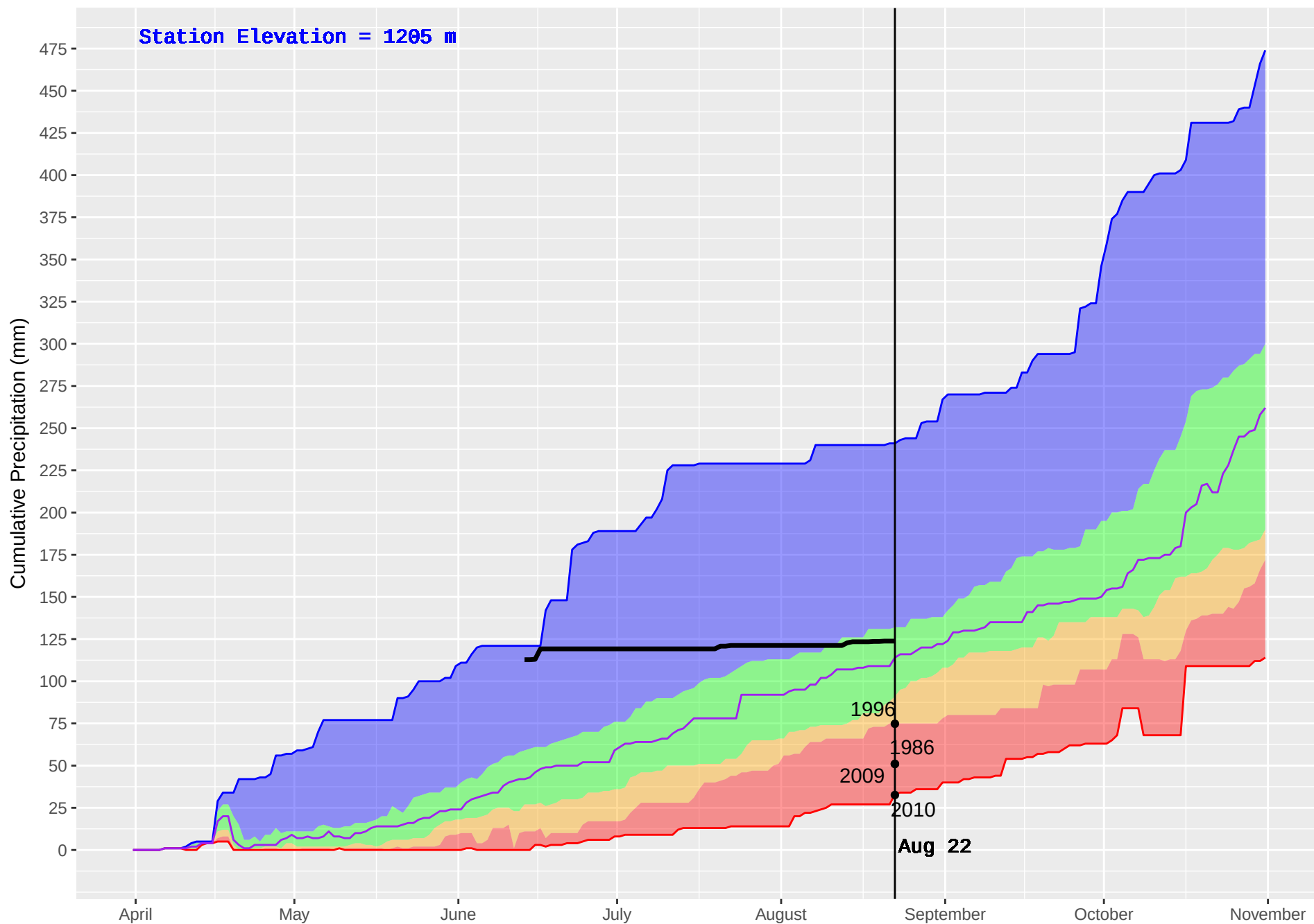
GWYNETH LAKE (309) : Historical (1986–2016) and Current (2017) Noon Cumulative Precipitation
