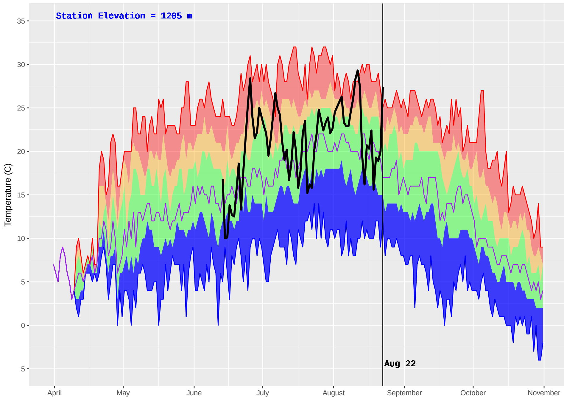
GWYNETH LAKE (309) : Historical (1986–2016) and Current (2017) Noon Temperature
