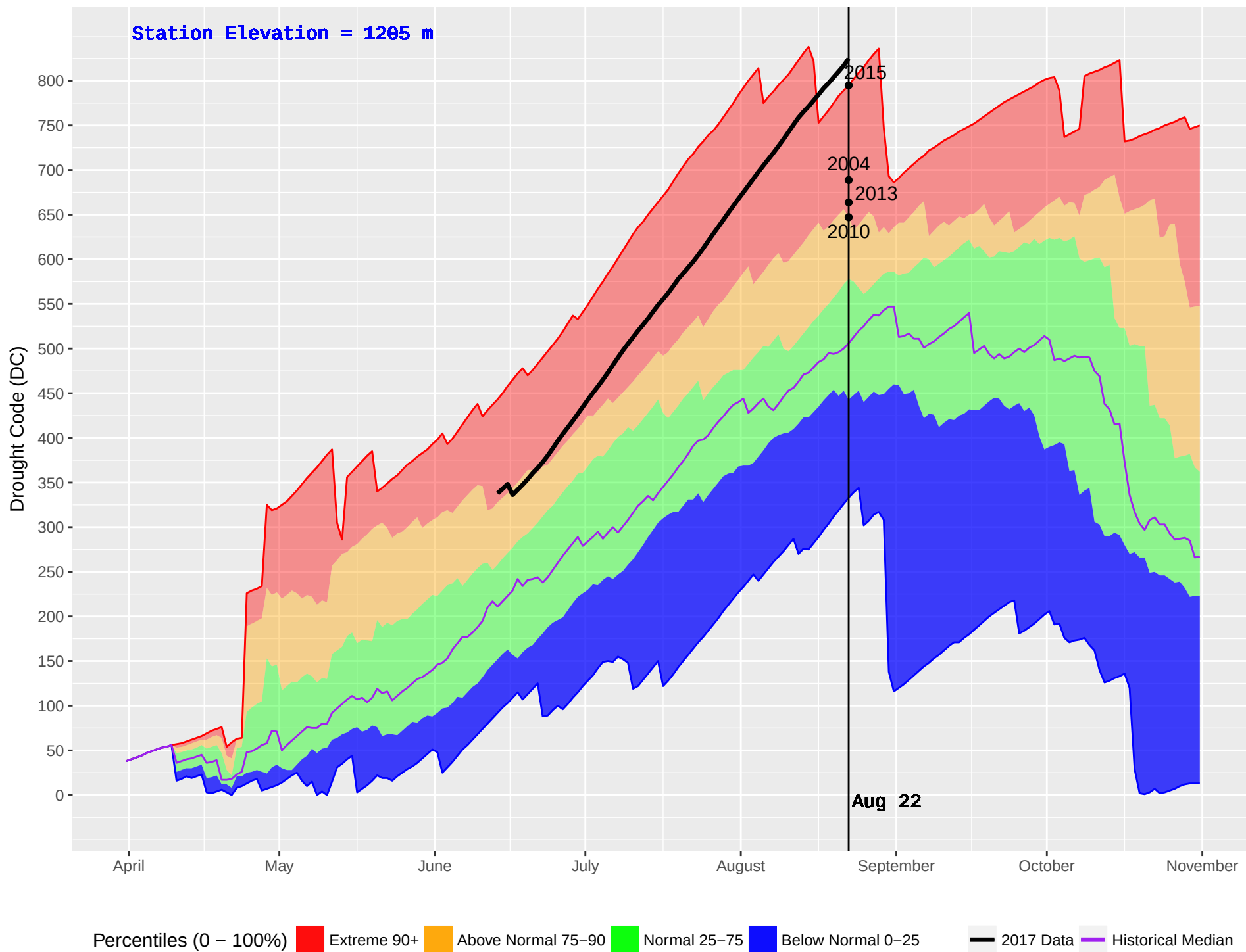
GWYNETH LAKE (309) : Historical (1986–2016) and Current (2017) Noon Drought Code (DC)
