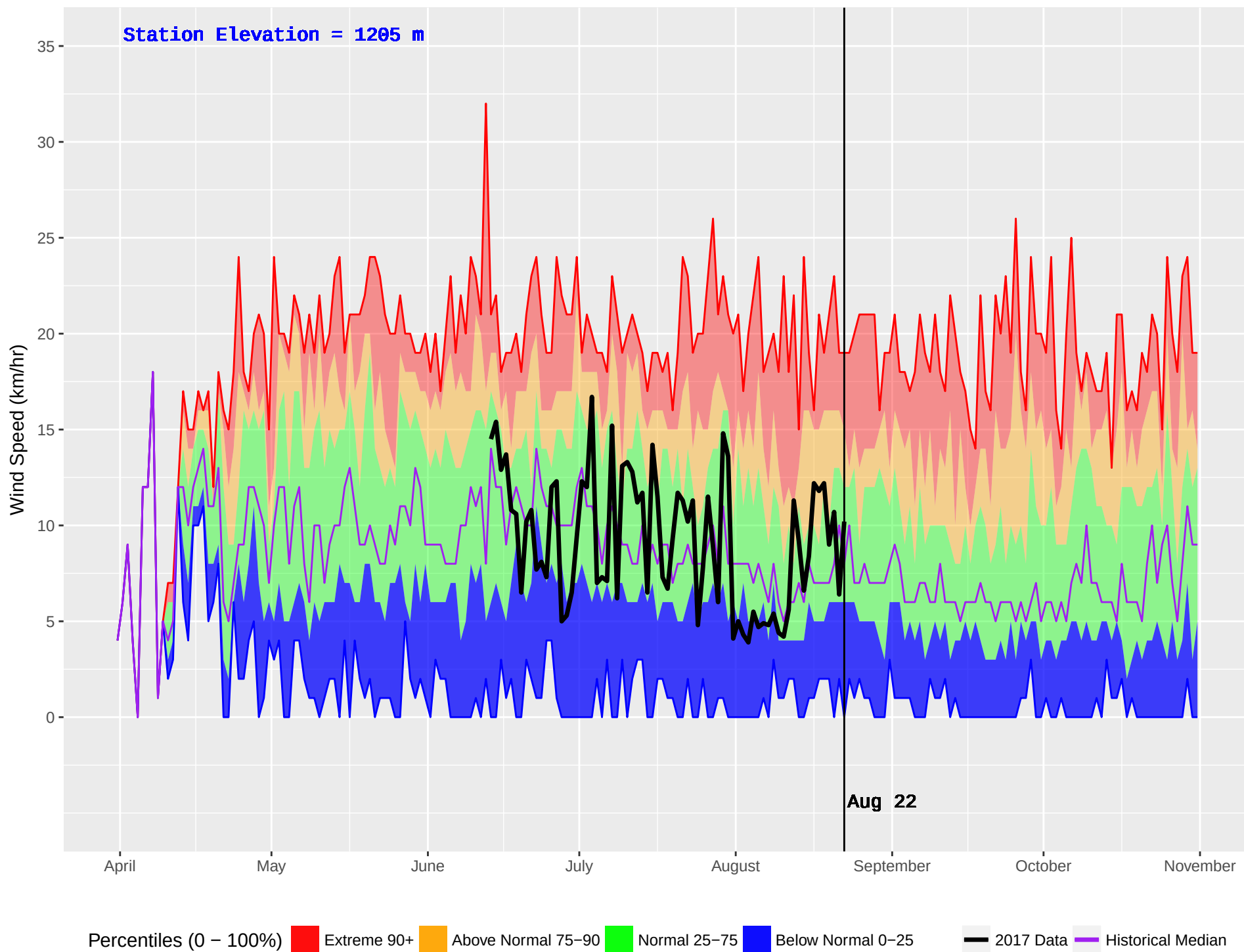
GWYNETH LAKE (309) : Historical (1986–2016) and Current (2017) Noon Wind Speed
