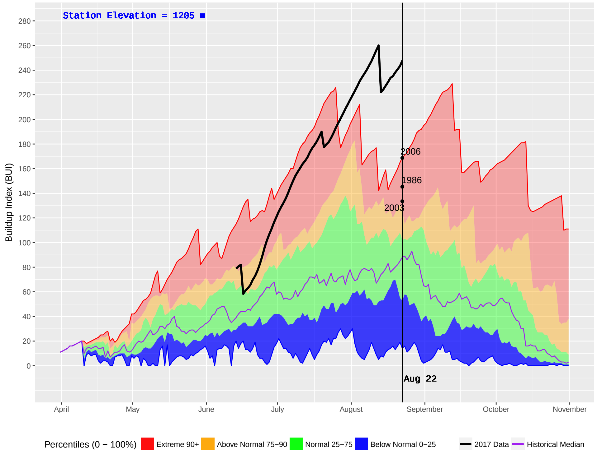
GWYNETH LAKE (309) : Historical (1986–2016) and Current (2017) Noon Buildup Index (BUI)
